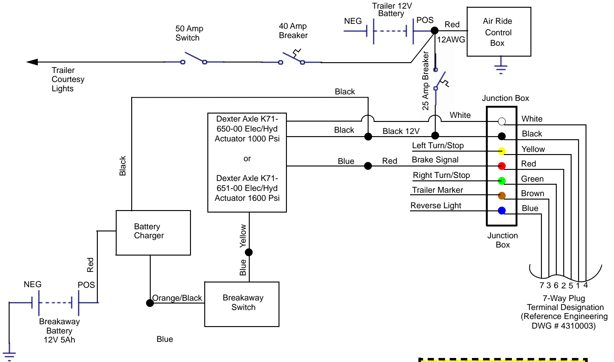
Trailer Junction Box Wiring Schematic Elec/Hyd Brake & Air Ride w/single hot wire.
